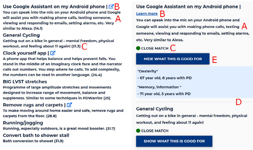
Fig. 3. Accessibility improvements to user interface (UI) of the PDCareBox — original (left) compared to updated (right). The updates include (A) increasing text line-height from 1.2 to 1.5, (B) text in place of icons, (C) more understandable goodness-of-fit visual indicator, (D) a thematic break, and (E) ‘Show what this is good for’-section that contains reflections from the users who rated the particular self-care technique.
